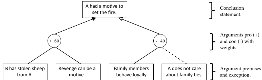
Figure 1. The arson example argument in the current Carneades visualization method.
