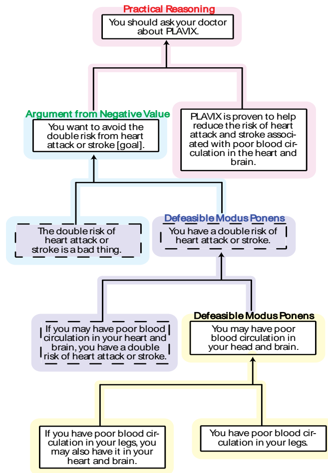
Figure 7: Argument Diagram of the PLAVIX Example
